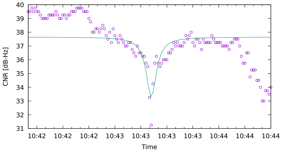
CNR fit for G01 on XiaomiMi8 - drive 1 (DOY262)
