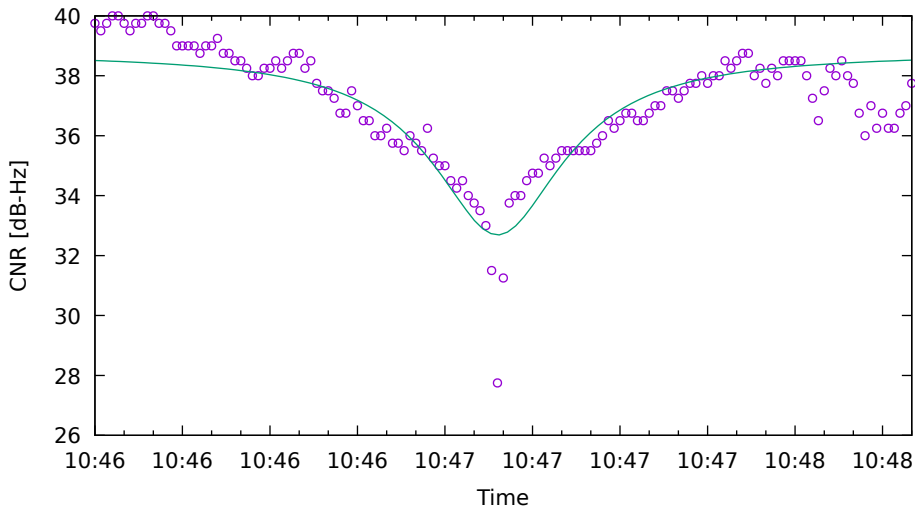
CNR fit for G01 on XiaomiMi8 - drive 3 (DOY262)
