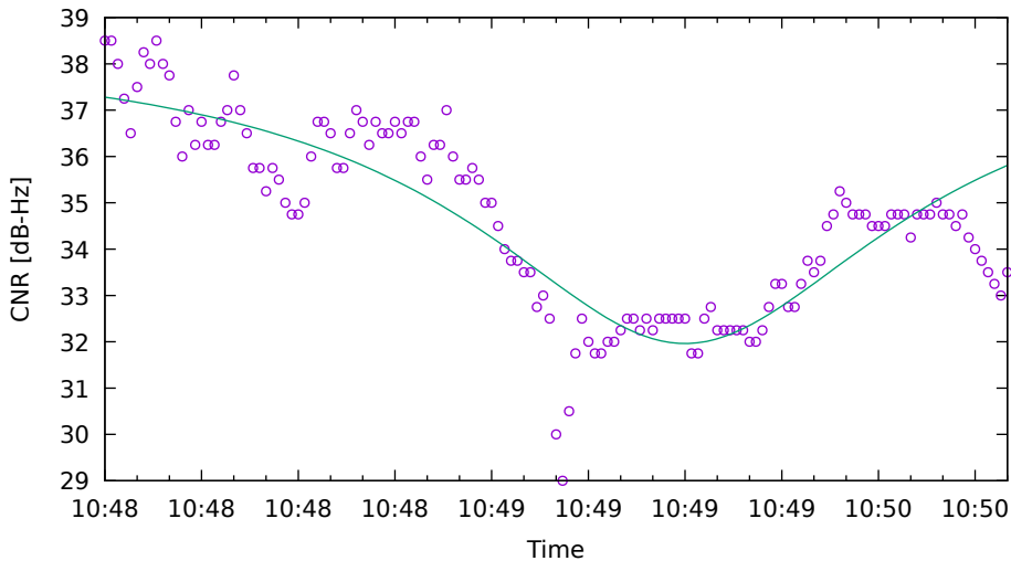
CNR fit for G01 on XiaomiMi8 - drive 4 (DOY262)
