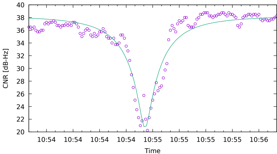
CNR fit for G01 on XiaomiMi8 - drive 7 (DOY262)
