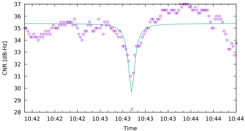
CNR fit for G04 on XiaomiMi8 - drive 1 (DOY262)
