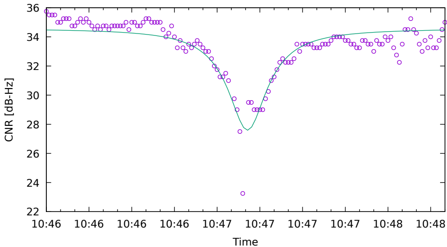
CNR fit for G04 on XiaomiMi8 - drive 3 (DOY262)
