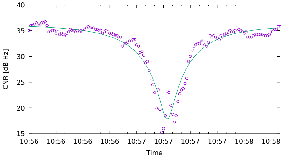
CNR fit for G04 on XiaomiMi8 - drive 8 (DOY262)
