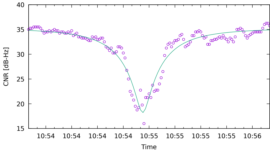
CNR fit for G22 on XiaomiMi8 - drive 7 (DOY262)
