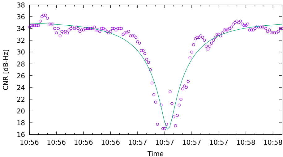
CNR fit for G22 on XiaomiMi8 - drive 8 (DOY262)
