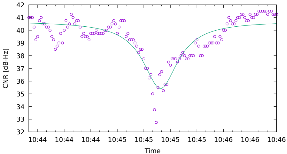
CNR fit for G31 on XiaomiMi8 - drive 2 (DOY262)
