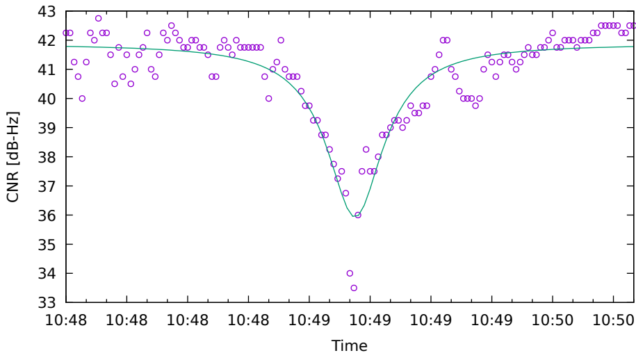
CNR fit for G31 on XiaomiMi8 - drive 4 (DOY262)
