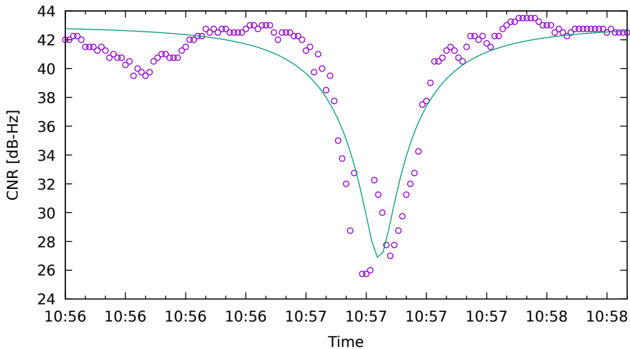
CNR fit for G31 on XiaomiMi8 - drive 8 (DOY262)
