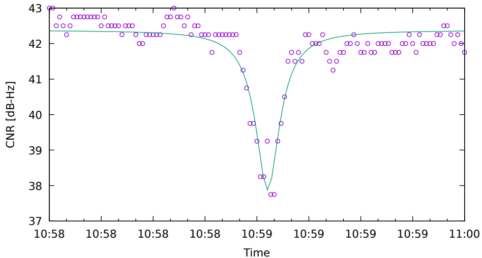
CNR fit for G31 on XiaomiMi8 - drive 9 (DOY262)
