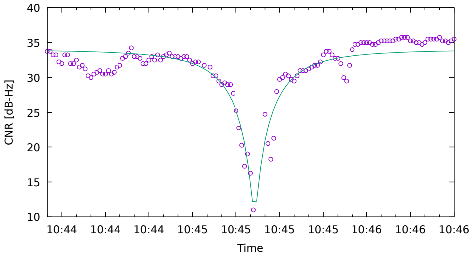
CNR fit for R01 on XiaomiMi8 - drive 2 (DOY262)
