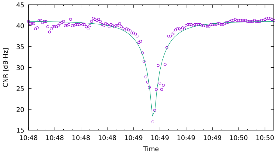
CNR fit for R08 on XiaomiMi8 - drive 4 (DOY262)
