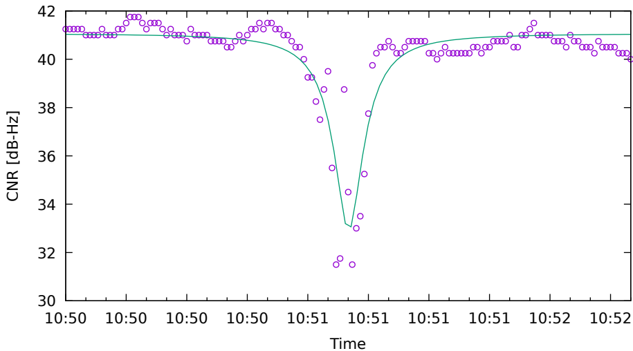
CNR fit for R08 on XiaomiMi8 - drive 5 (DOY262)
