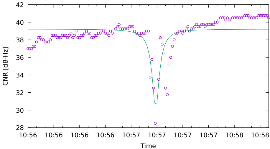
CNR fit for R08 on XiaomiMi8 - drive 8 (DOY262)
