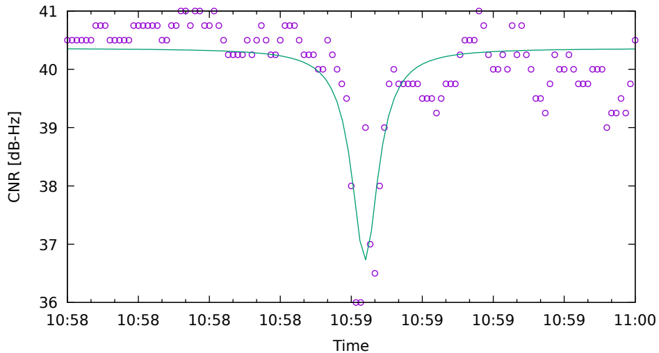
CNR fit for R08 on XiaomiMi8 - drive 9 (DOY262)
