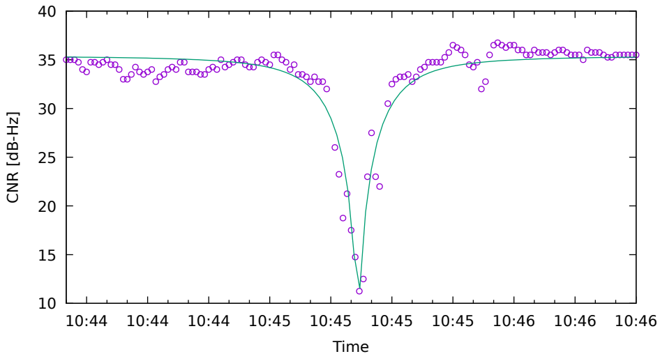
CNR fit for R23 on XiaomiMi8 - drive 2 (DOY262)
