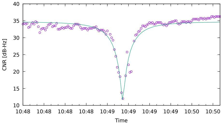
CNR fit for R23 on XiaomiMi8 - drive 4 (DOY262)
