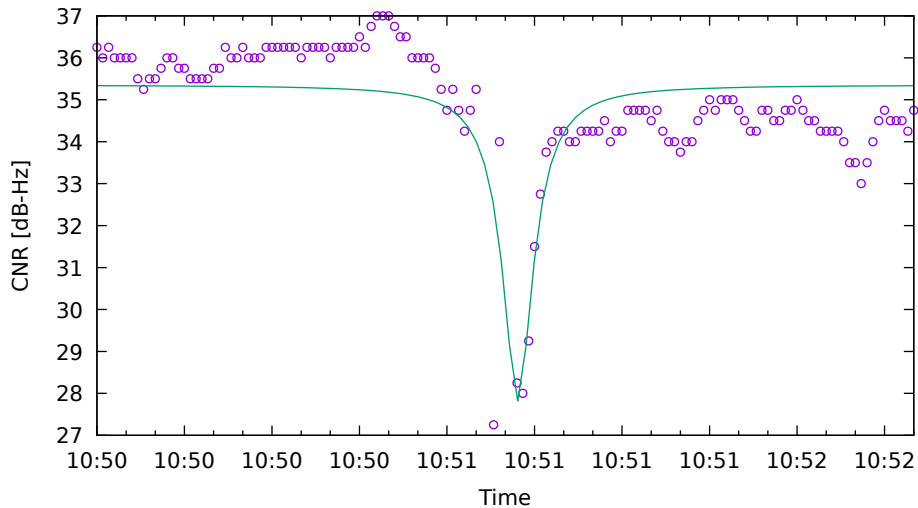
CNR fit for R24 on XiaomiMi8 - drive 5 (DOY262)
