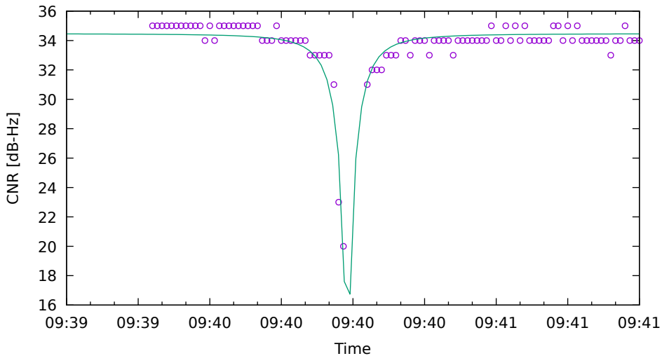
CNR fit for C05 on HuaweiP40 - drive 1 (DOY263)
