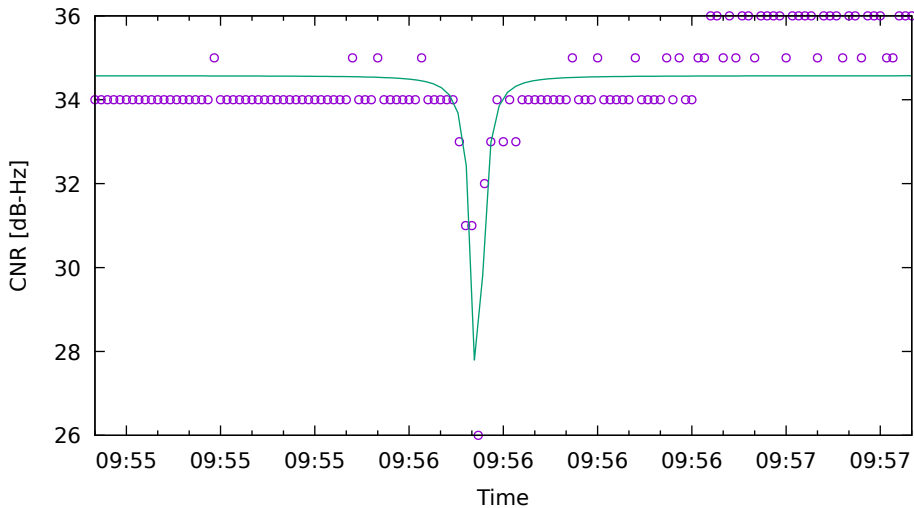
CNR fit for C05 on HuaweiP40 - drive 10 (DOY263)
