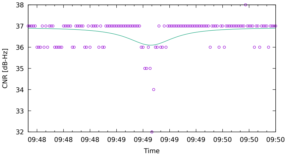
CNR fit for C05 on HuaweiP40 - drive 6 (DOY263)
