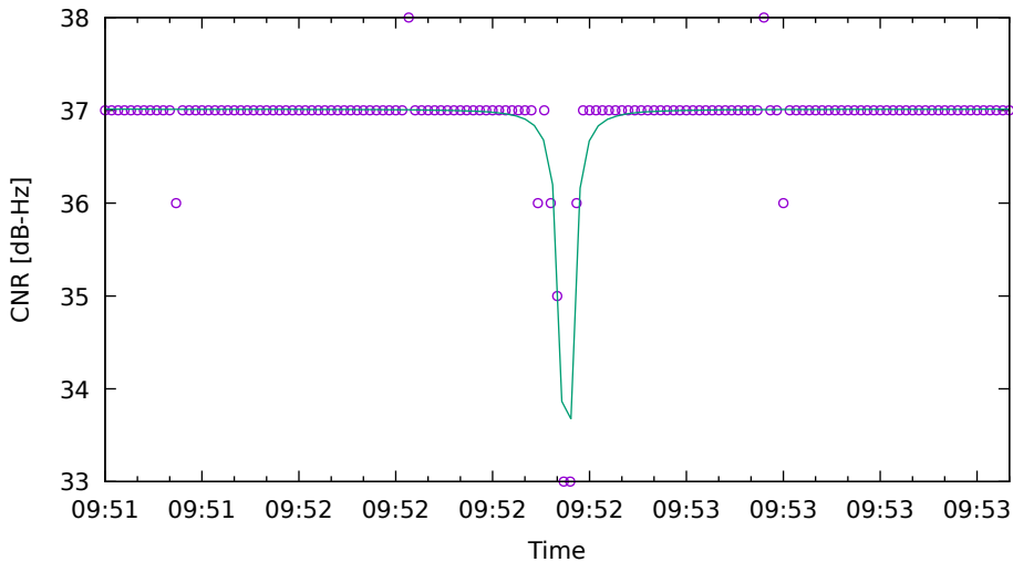
CNR fit for C05 on HuaweiP40 - drive 8 (DOY263)
