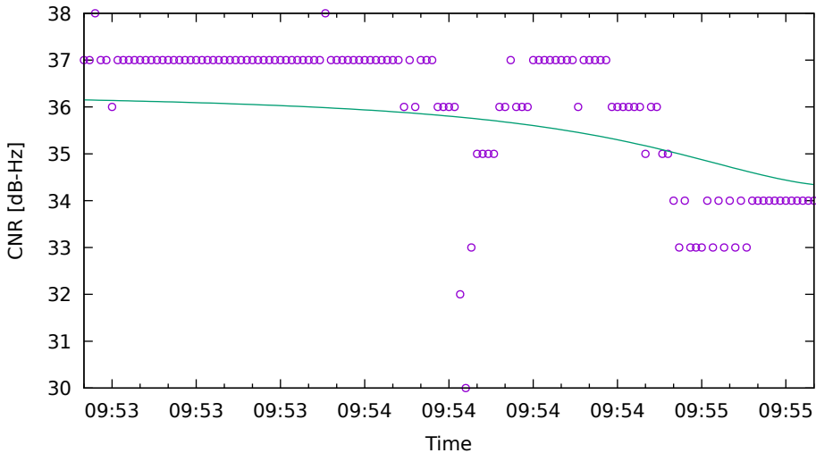
CNR fit for C05 on HuaweiP40 - drive 9 (DOY263)
