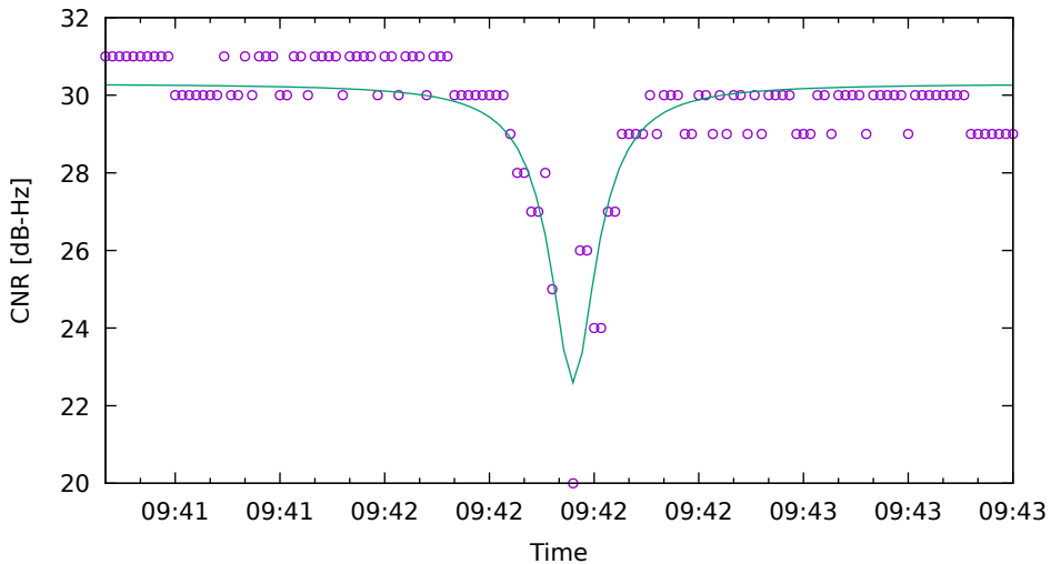
CNR fit for C06 on HuaweiP40 - drive 2 (DOY263)
