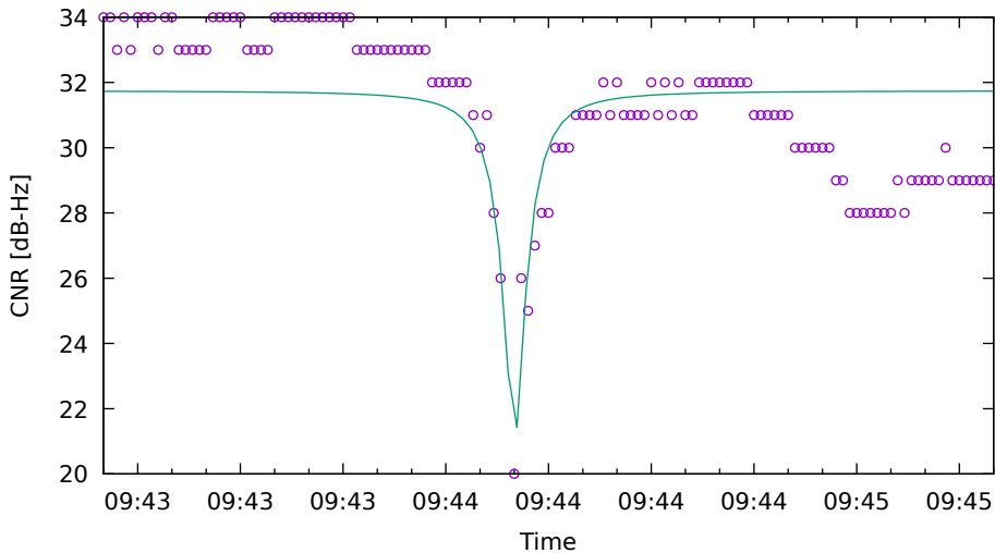
CNR fit for C11 on HuaweiP40 - drive 3 (DOY263)
