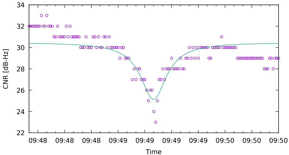
CNR fit for C11 on HuaweiP40 - drive 6 (DOY263)
