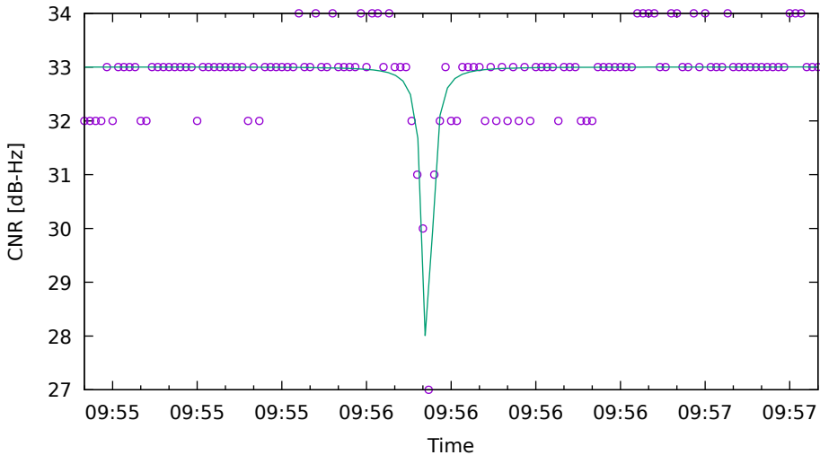
CNR fit for C16 on HuaweiP40 - drive 10 (DOY263)
