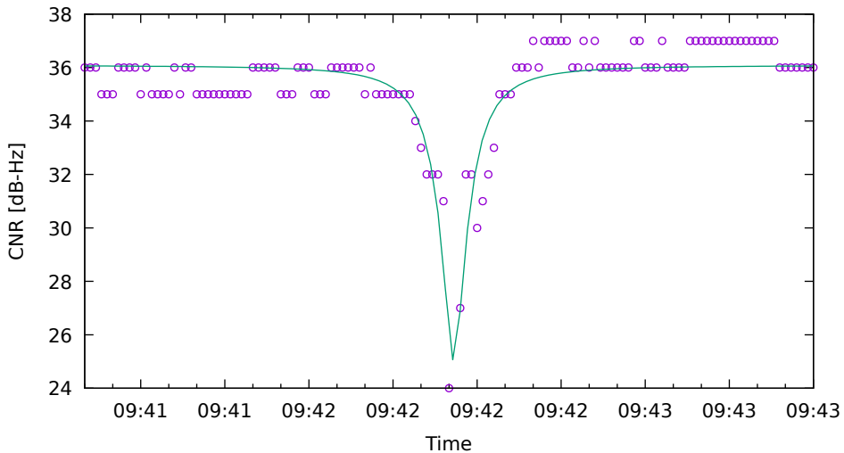
CNR fit for C16 on HuaweiP40 - drive 2 (DOY263)
