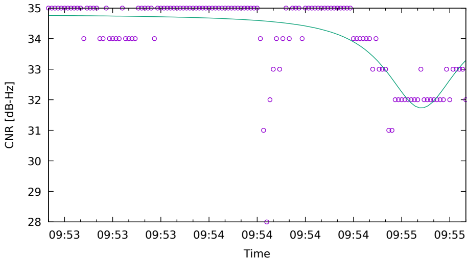
CNR fit for C16 on HuaweiP40 - drive 9 (DOY263)
