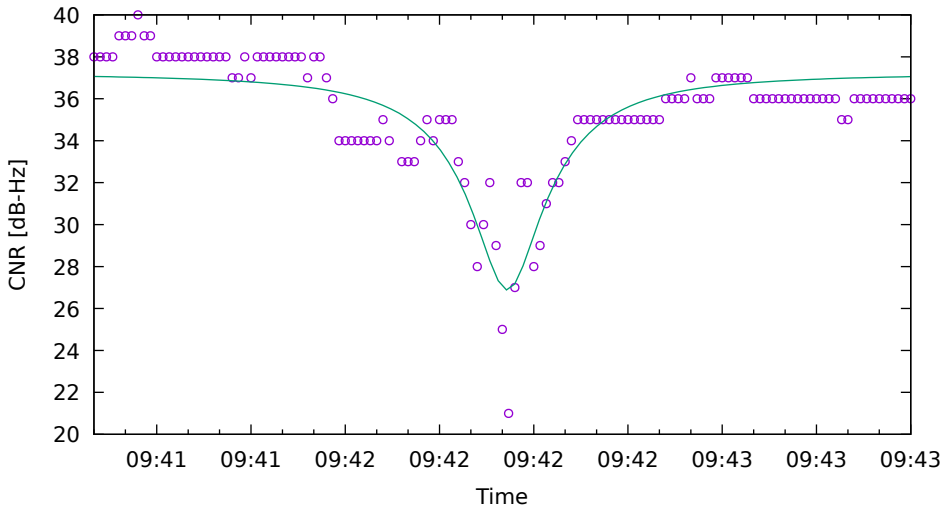
CNR fit for G01 on HuaweiP40 - drive 2 (DOY263)
