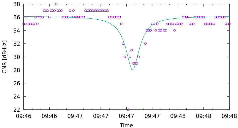
CNR fit for G01 on HuaweiP40 - drive 5 (DOY263)
