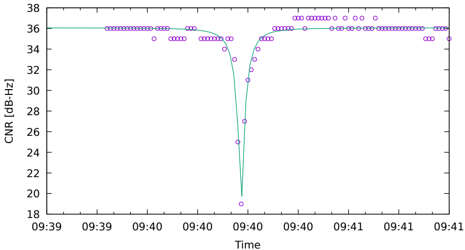
CNR fit for G04 on HuaweiP40 - drive 1 (DOY263)
