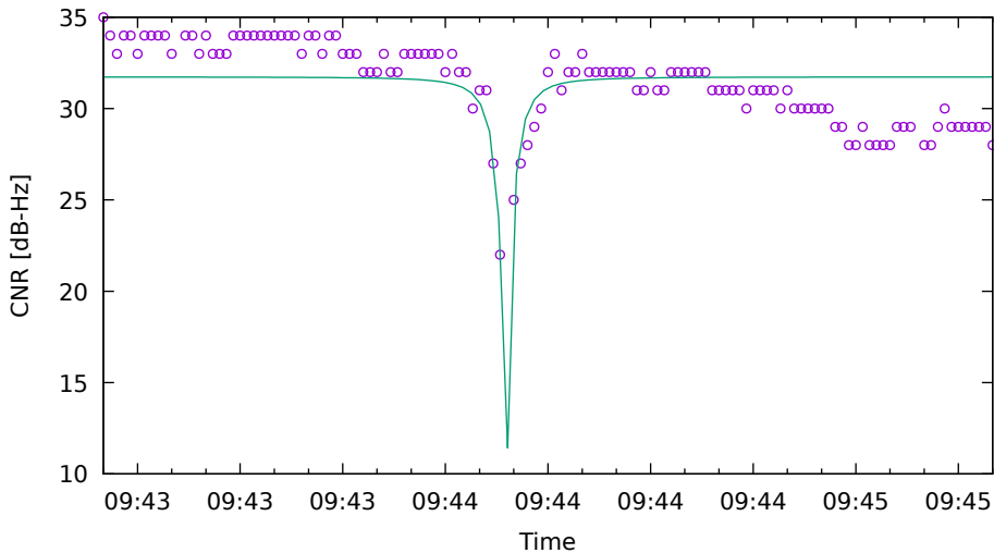
CNR fit for G08 on HuaweiP40 - drive 3 (DOY263)
