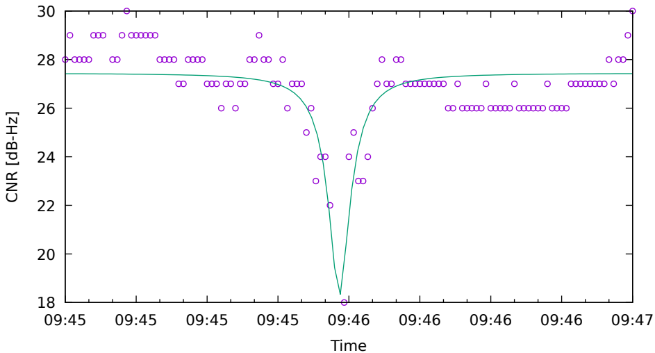
CNR fit for G08 on HuaweiP40 - drive 4 (DOY263)
