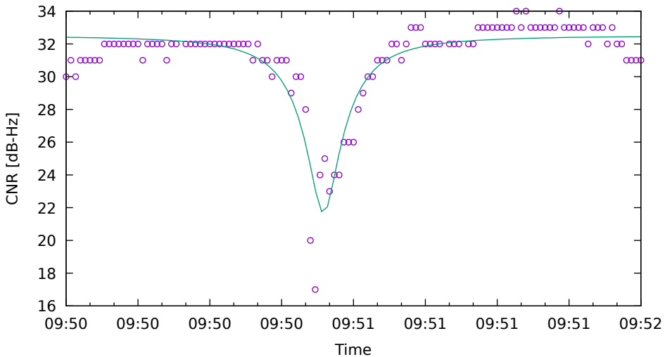
CNR fit for G08 on HuaweiP40 - drive 7 (DOY263)
