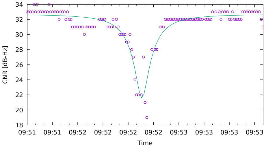
CNR fit for G08 on HuaweiP40 - drive 8 (DOY263)
