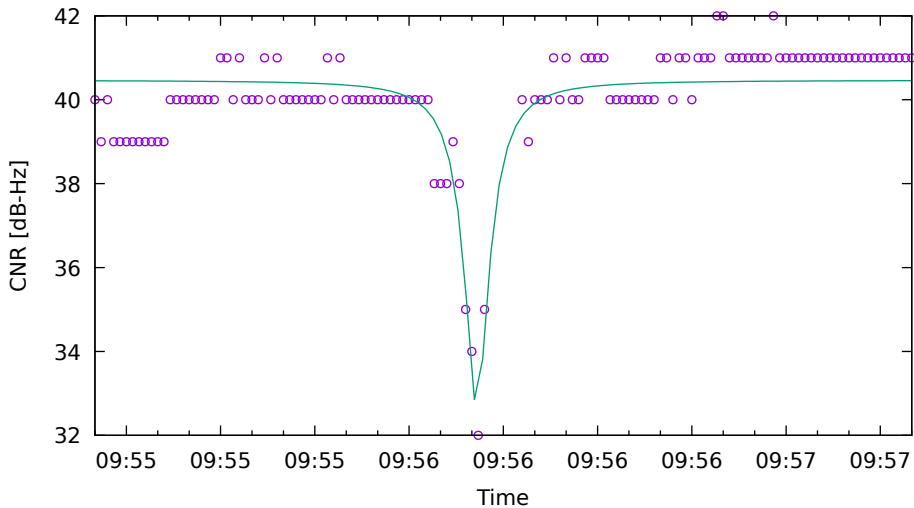
CNR fit for G17 on HuaweiP40 - drive 10 (DOY263)
