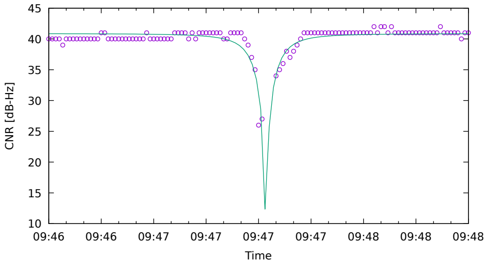
CNR fit for G17 on HuaweiP40 - drive 5 (DOY263)
