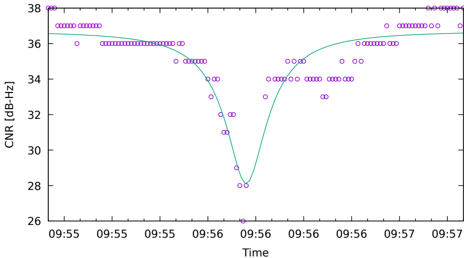
CNR fit for G21 on HuaweiP40 - drive 10 (DOY263)
