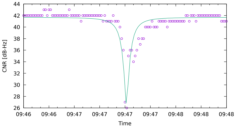
CNR fit for G21 on HuaweiP40 - drive 5 (DOY263)
