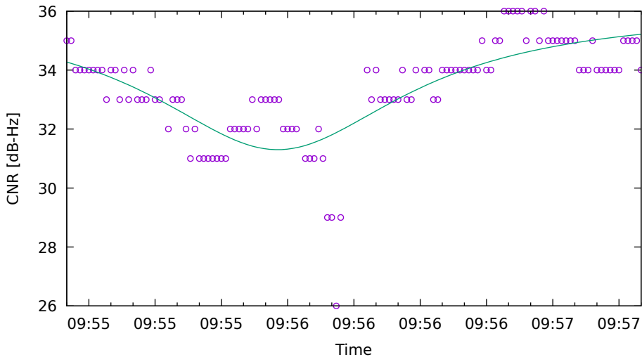
CNR fit for G22 on HuaweiP40 - drive 10 (DOY263)
