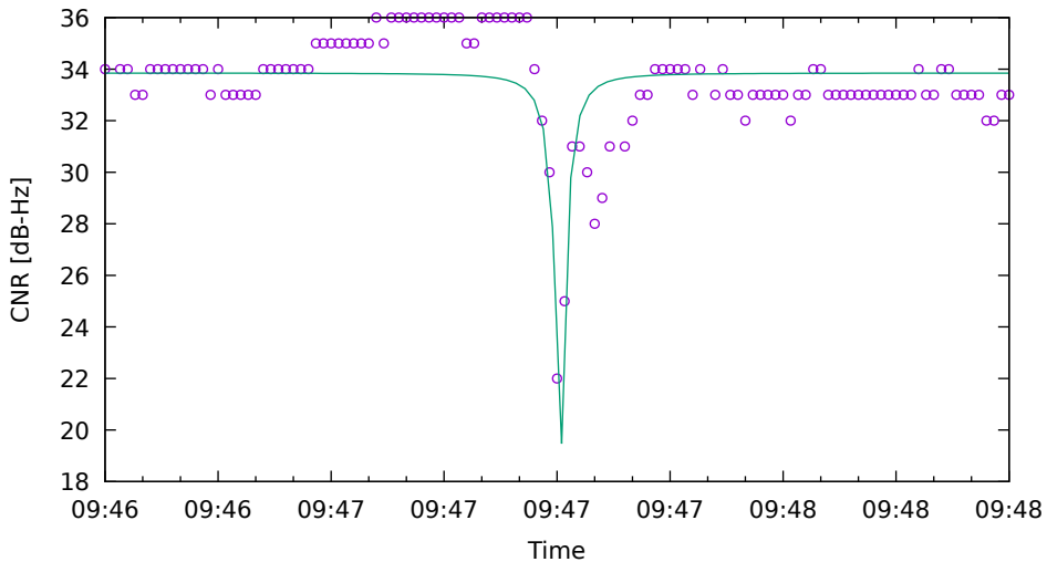
CNR fit for G22 on HuaweiP40 - drive 5 (DOY263)
