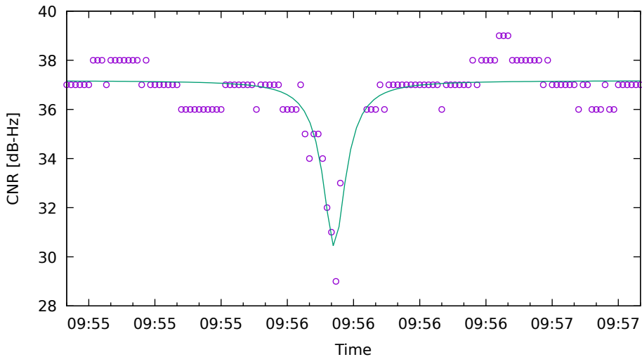
CNR fit for G31 on HuaweiP40 - drive 10 (DOY263)
