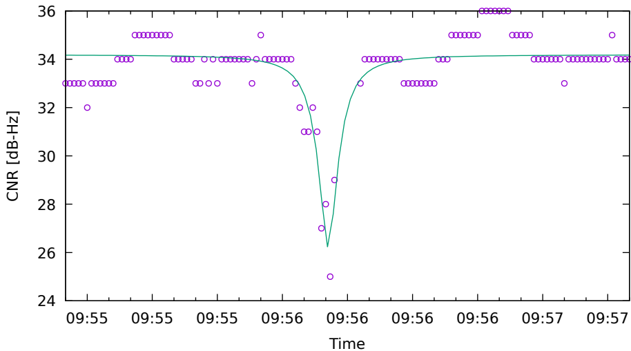
CNR fit for G32 on HuaweiP40 - drive 10 (DOY263)
