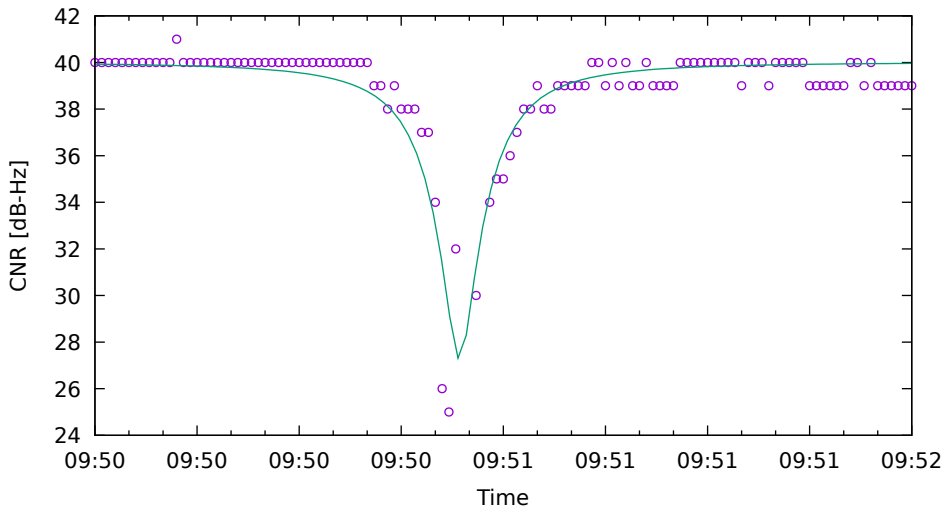
CNR fit for G32 on HuaweiP40 - drive 7 (DOY263)
