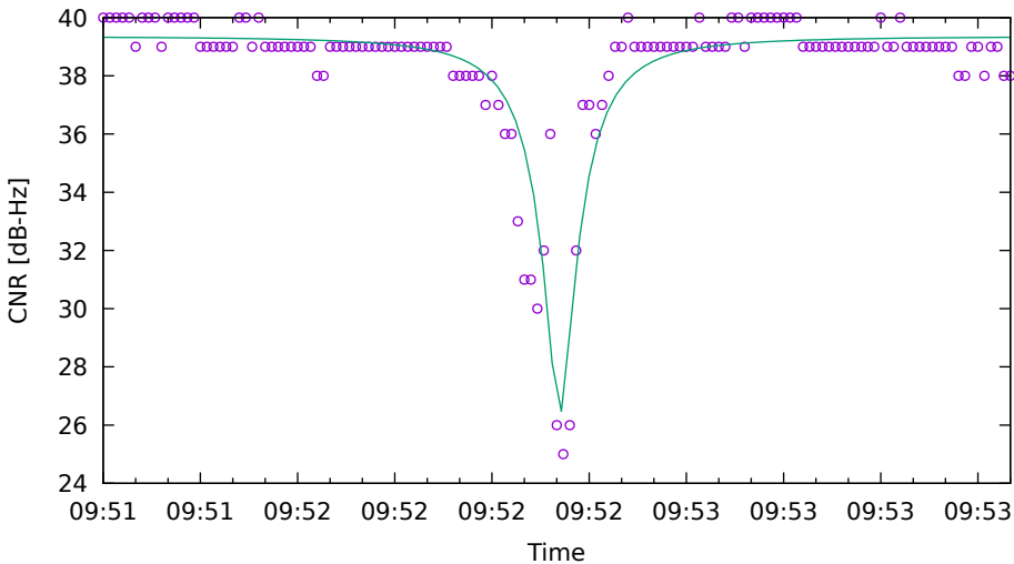
CNR fit for G32 on HuaweiP40 - drive 8 (DOY263)
