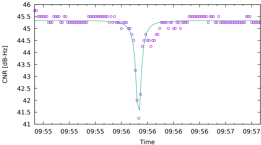
CNR fit for C05 on SamsungS20 - drive 10 (DOY263)
